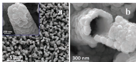
Figure 1. (a) SEM image of Pt-Ni-P NTAs after etching ZnO nanorods and (b) typical SEM image of a broken Pt-Ni-P nanotube.
